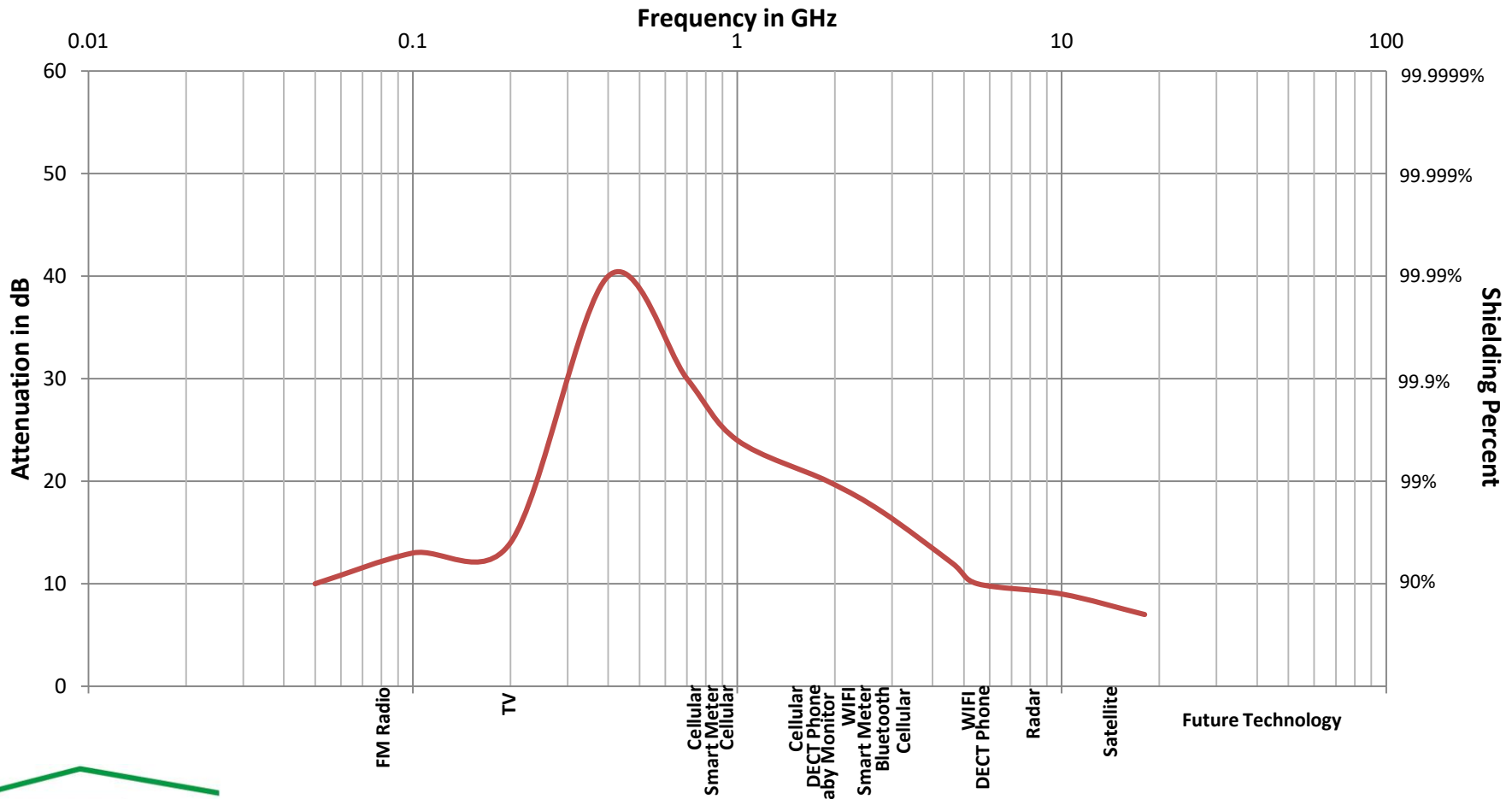
Swiss Shield Daylite Bed Canopy RF Shielding Performance
